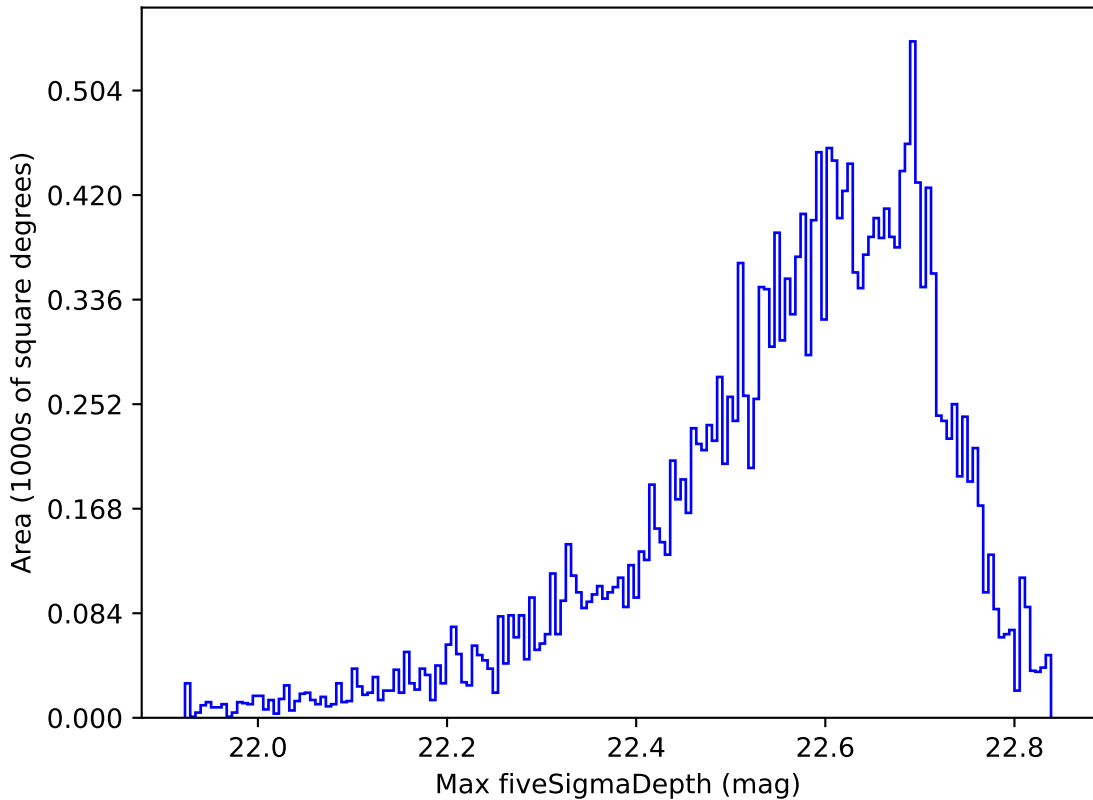
weather_cloudso16v3.4_10yrs All sky y band: Max fiveSigmaDepth
