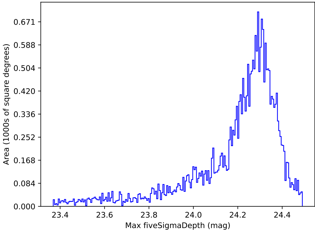
weather_cloudso16v3.4_10yrs All sky i band: Max fiveSigmaDepth
