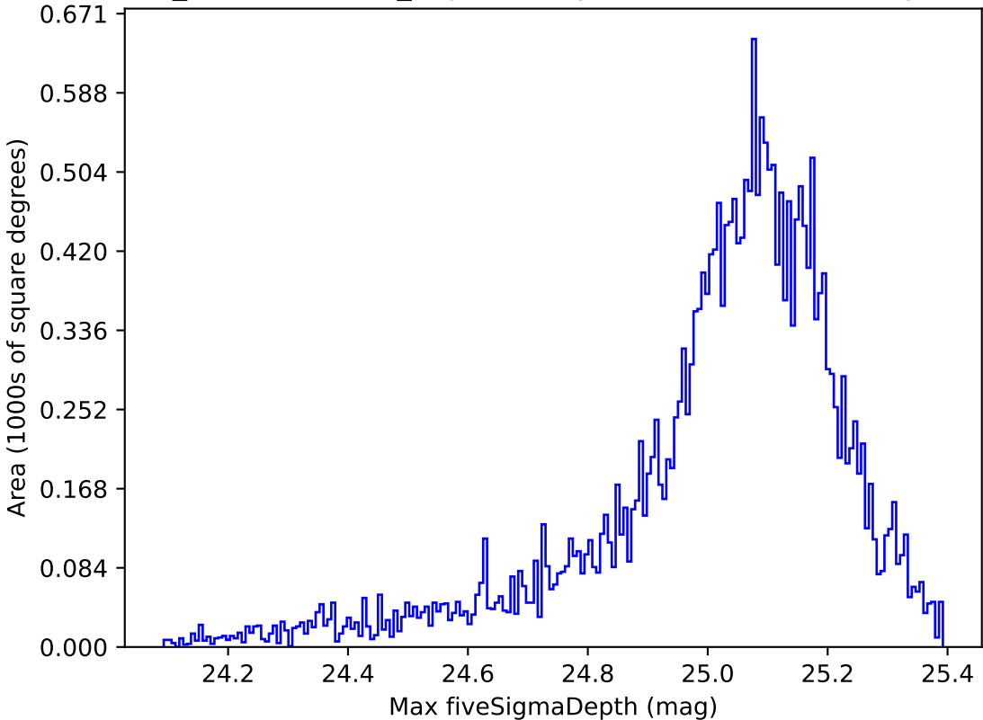
weather_cloudso16v3.4_10yrs All sky all bands: Max fiveSigmaDepth
