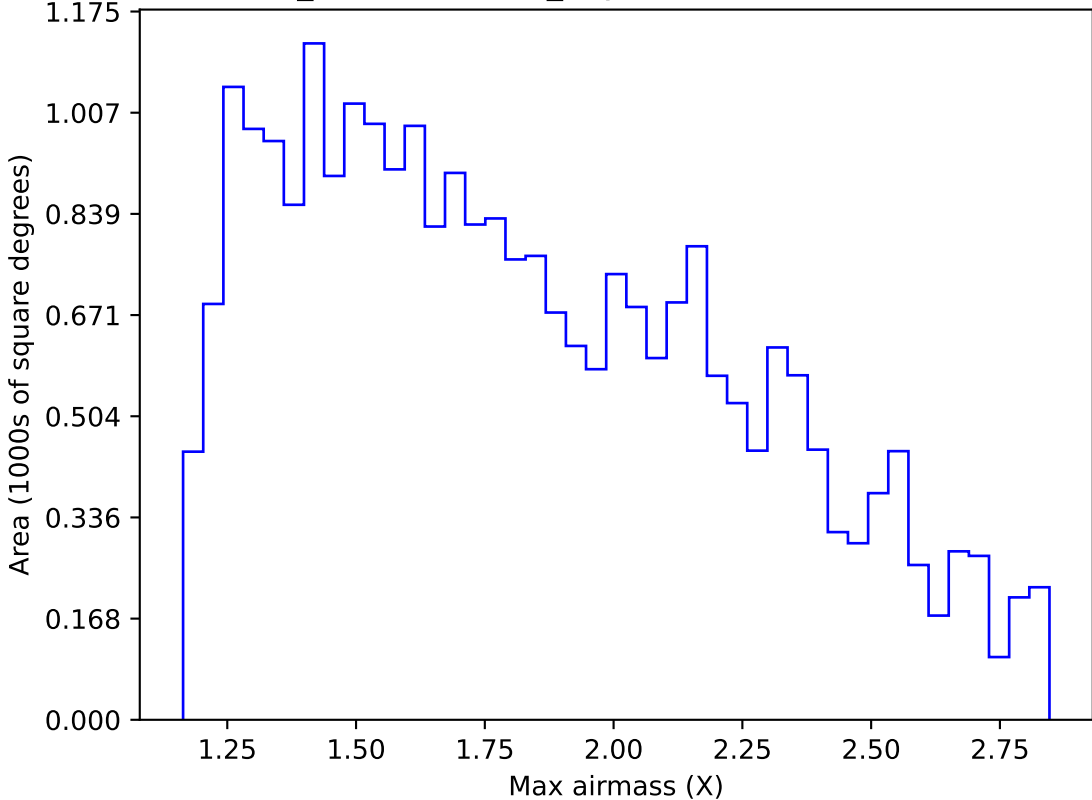
weather_cloudso16v3.4_10yrs Yr 1 z band: Max airmass
