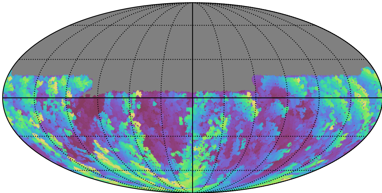
weather_cloudso16v3.4_10yrs Yr 1 y band: Max airmass
