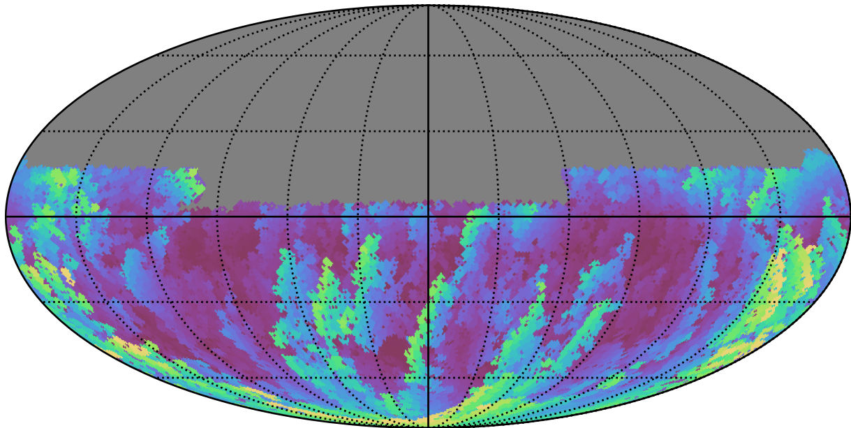
weather_cloudso16v3.4_10yrs Yr 1 u band: Max airmass
