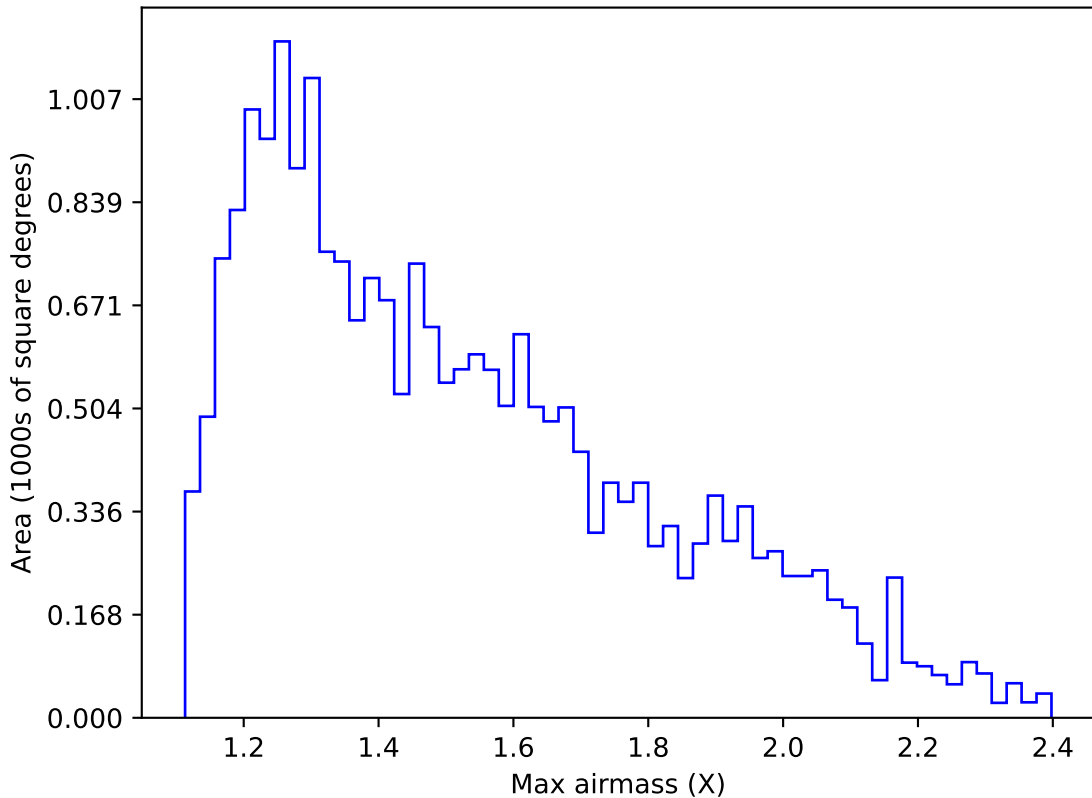
weather_cloudso16v3.4_10yrs Yr 1 u band: Max airmass
