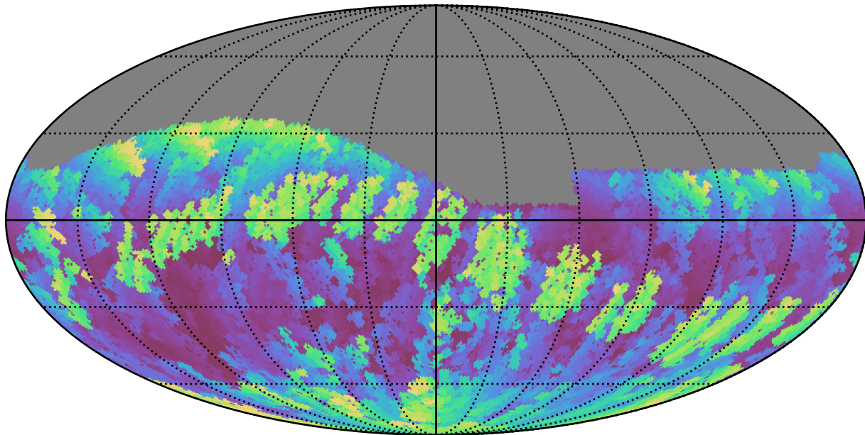
weather_cloudso16v3.4_10yrs Yr 1 r band: Max airmass
