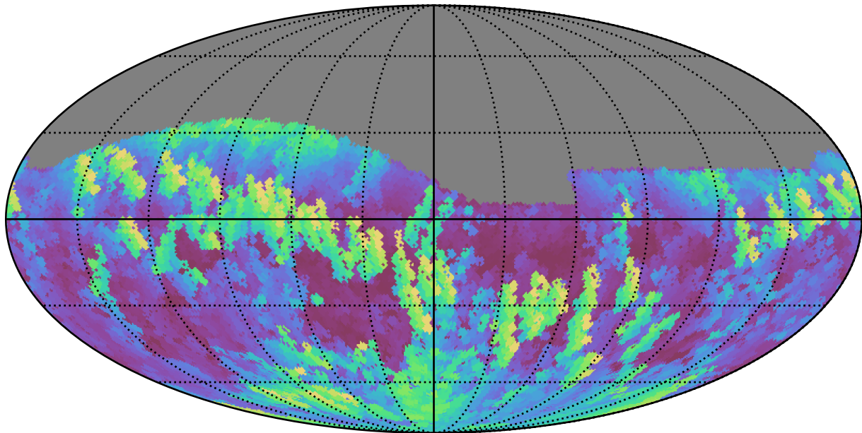
weather_cloudso16v3.4_10yrs Yr 1 i band: Max airmass
