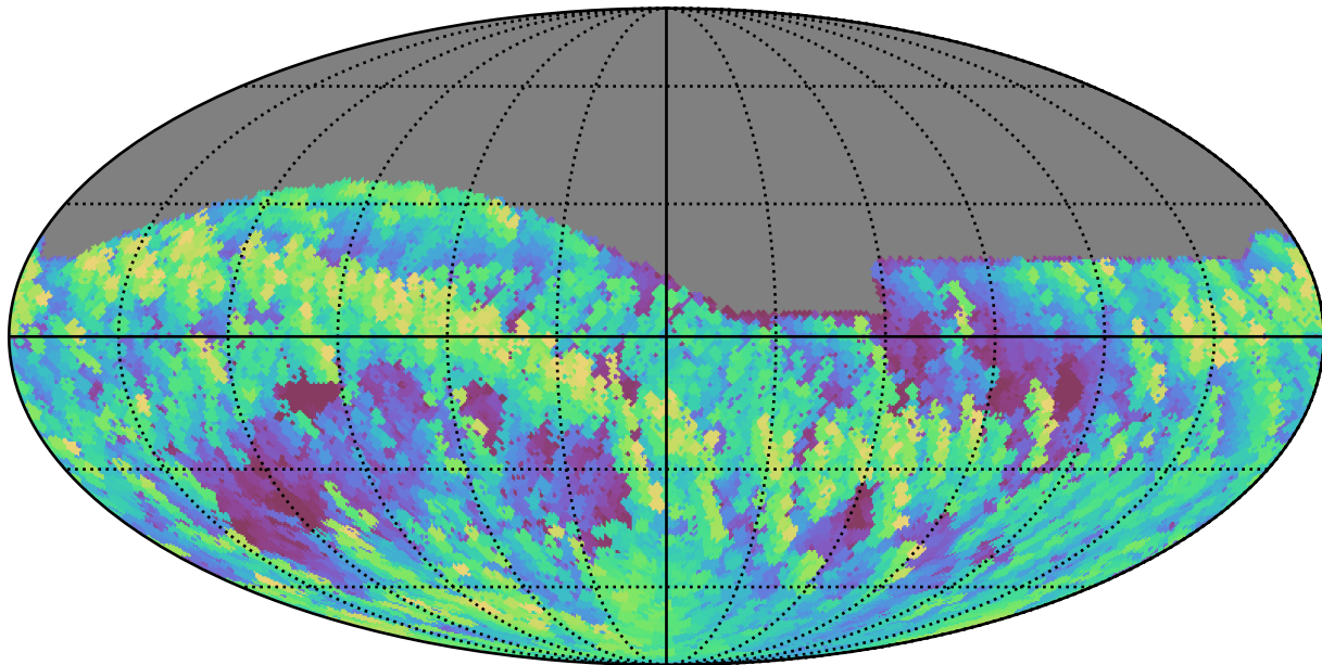
weather_cloudso16v3.4_10yrs Yr 1 all bands: Max airmass
