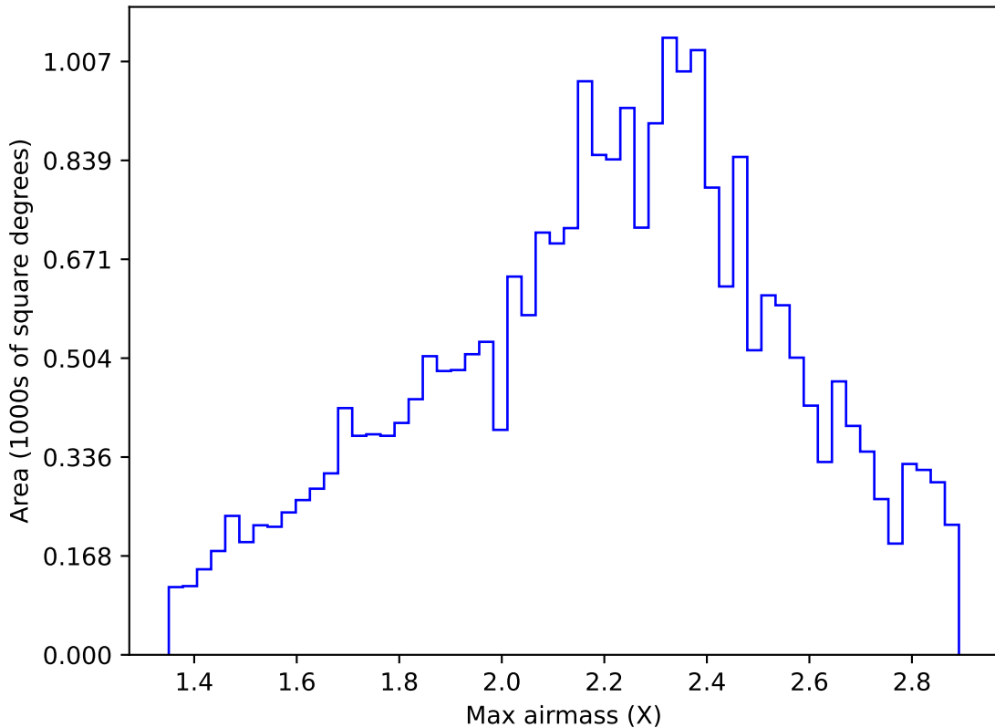
weather_cloudso16v3.4_10yrs Yr 1 all bands: Max airmass
