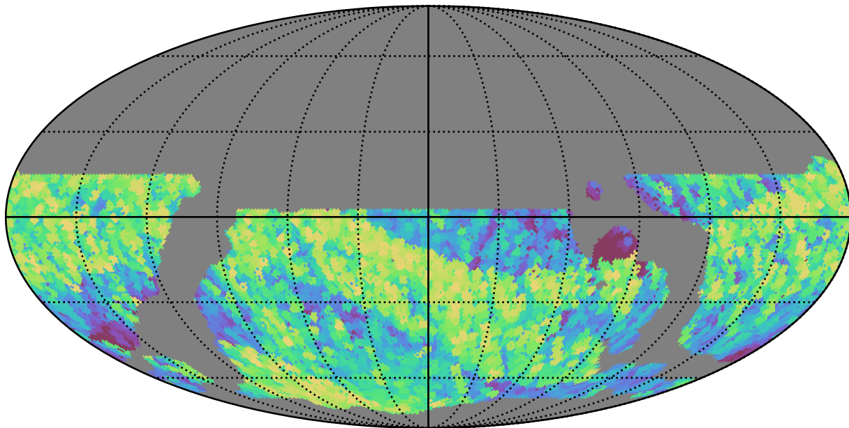
weather_cloudso16v3.4_10yrs WFD z band: Max airmass
