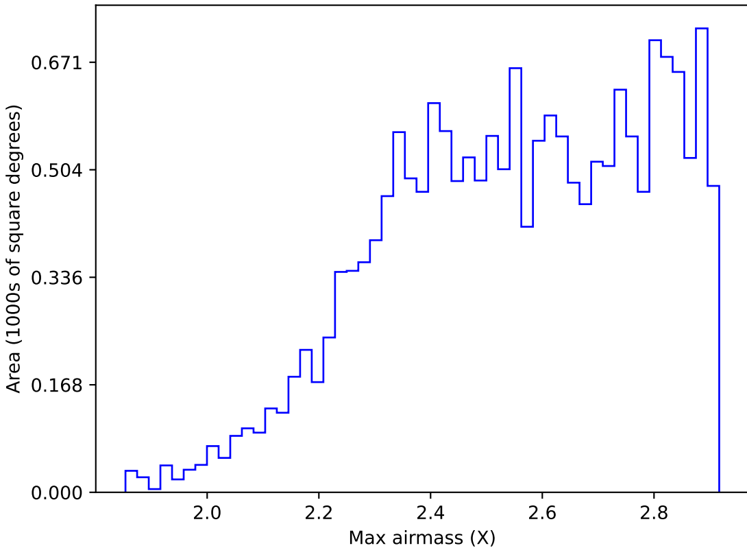
weather_cloudso16v3.4_10yrs WFD z band: Max airmass
