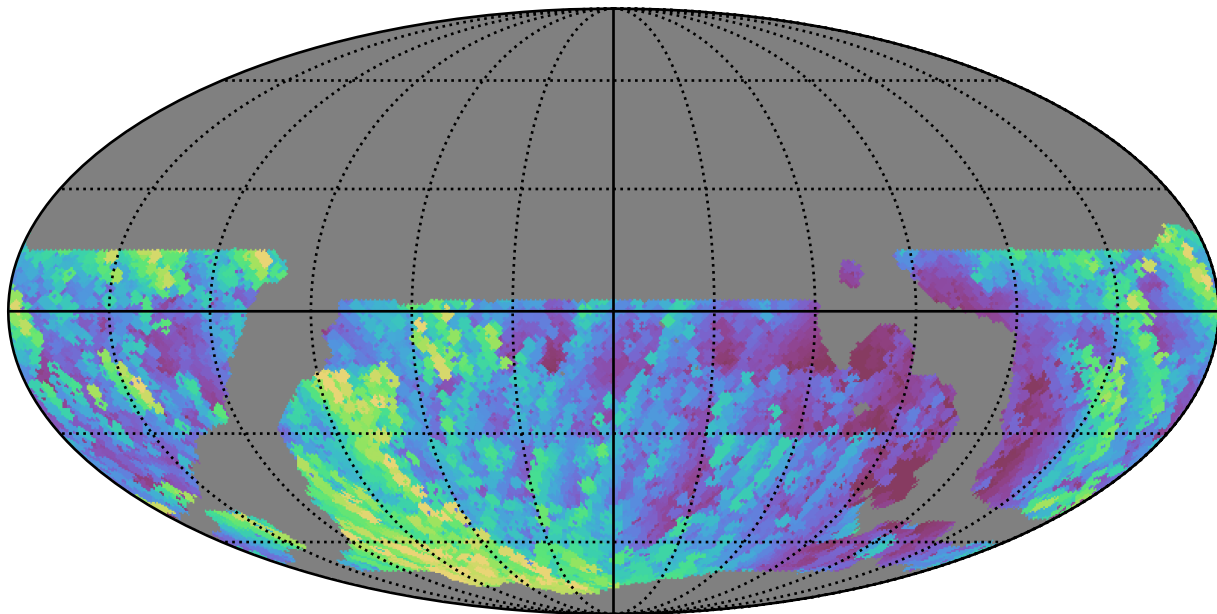
weather_cloudso16v3.4_10yrs WFD u band: Max airmass
