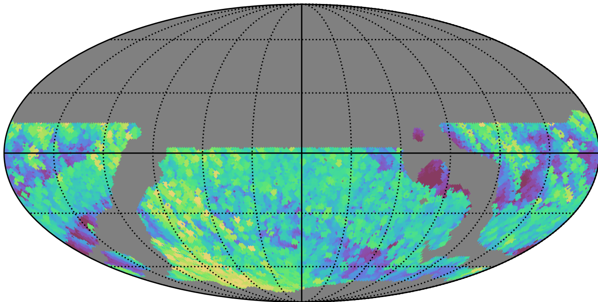
weather_cloudso16v3.4_10yrs WFD r band: Max airmass
