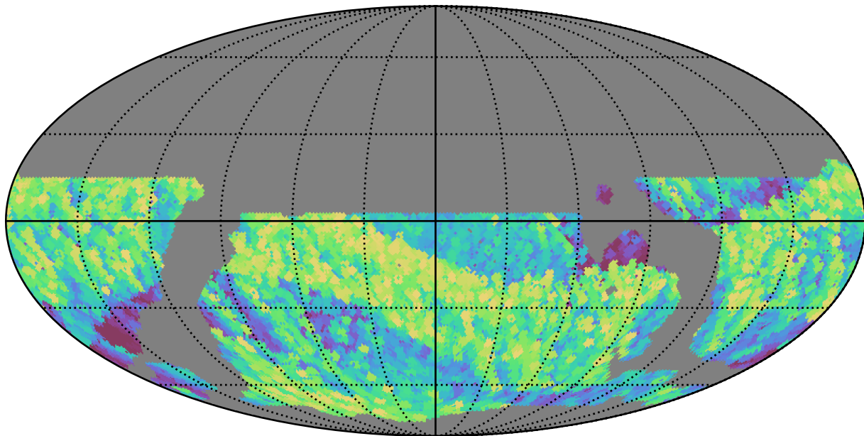
weather_cloudso16v3.4_10yrs WFD i band: Max airmass
