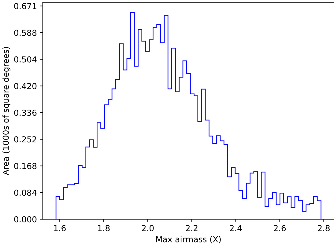
weather_cloudso16v3.4_10yrs WFD g band: Max airmass
