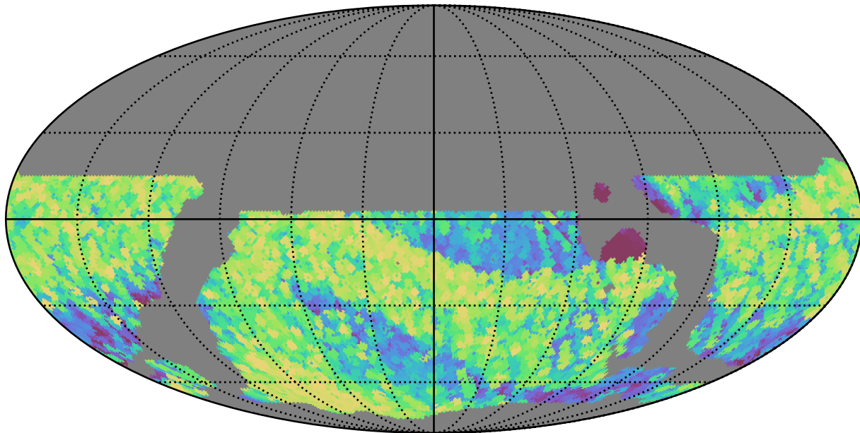
weather_cloudso16v3.4_10yrs WFD all bands: Max airmass
