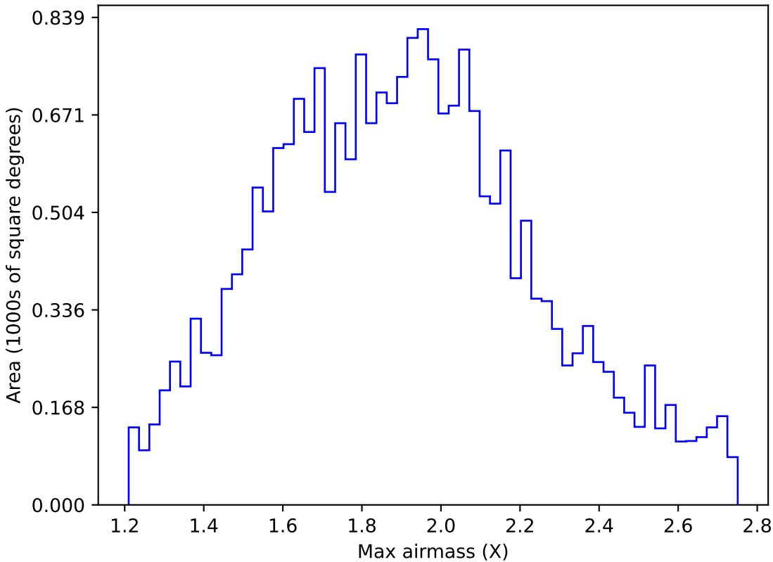
weather_cloudso16v3.4_10yrs All sky u band: Max airmass
