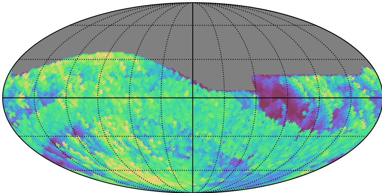
weather_cloudso16v3.4_10yrs All sky r band: Max airmass
