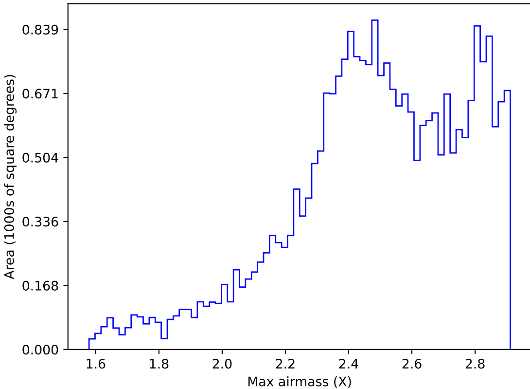
weather_cloudso16v3.4_10yrs All sky i band: Max airmass
