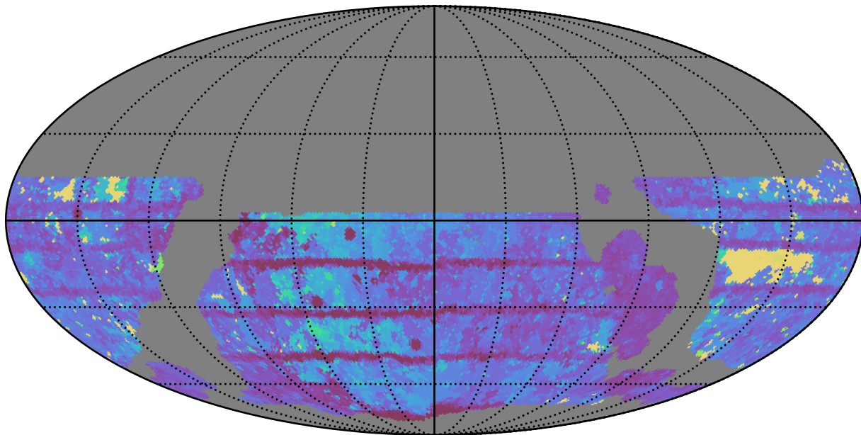
weather_cloudso16v3.4_10yrs WFD z band: Max Inter-Night Gap
