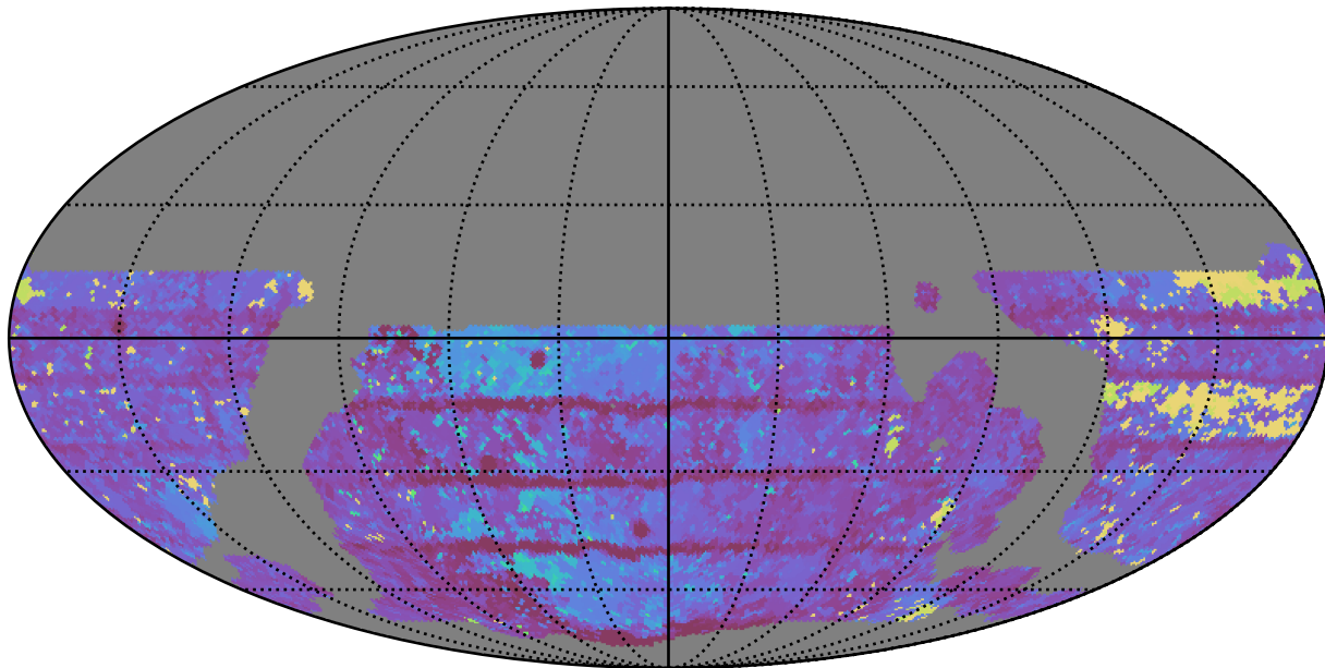
weather_cloudso16v3.4_10yrs WFD y band: Max Inter-Night Gap
