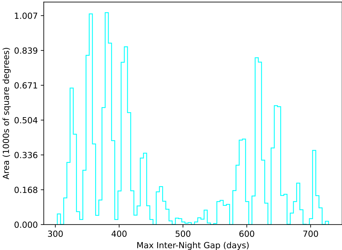
weather_cloudso16v3.4_10yrs WFD u band: Max Inter-Night Gap
