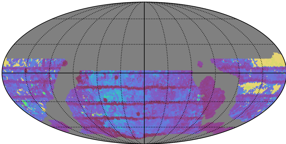
weather_cloudso16v3.4_10yrs WFD r band: Max Inter-Night Gap
