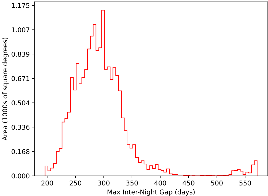
weather_cloudso16v3.4_10yrs WFD i band: Max Inter-Night Gap
