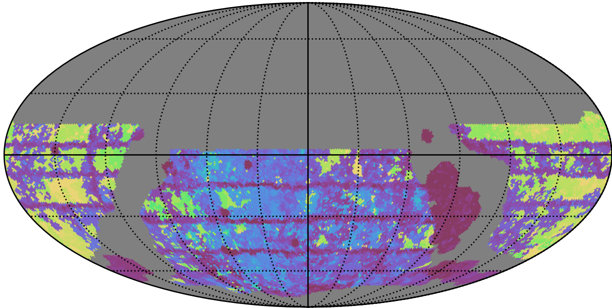
weather_cloudso16v3.4_10yrs WFD g band: Max Inter-Night Gap
