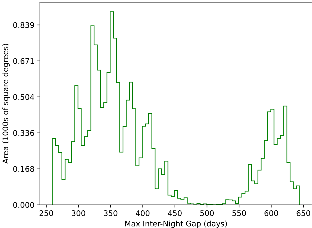
weather_cloudso16v3.4_10yrs WFD g band: Max Inter-Night Gap
