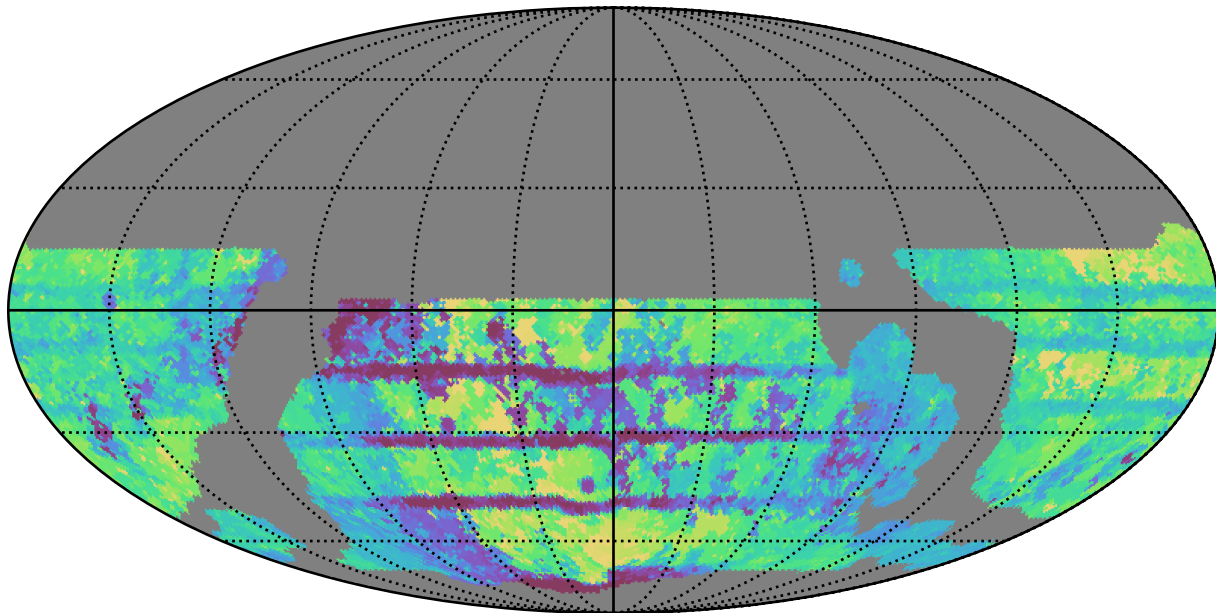
weather_cloudso16v3.4_10yrs WFD all bands: Max Inter-Night Gap
