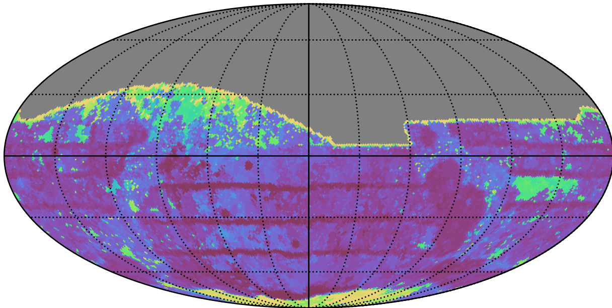
weather_cloudso16v3.4_10yrs All sky z band: Max Inter-Night Gap
