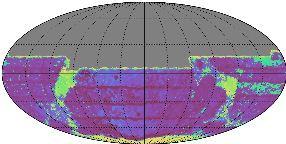
weather_cloudso16v3.4_10yrs All sky y band: Max Inter-Night Gap
