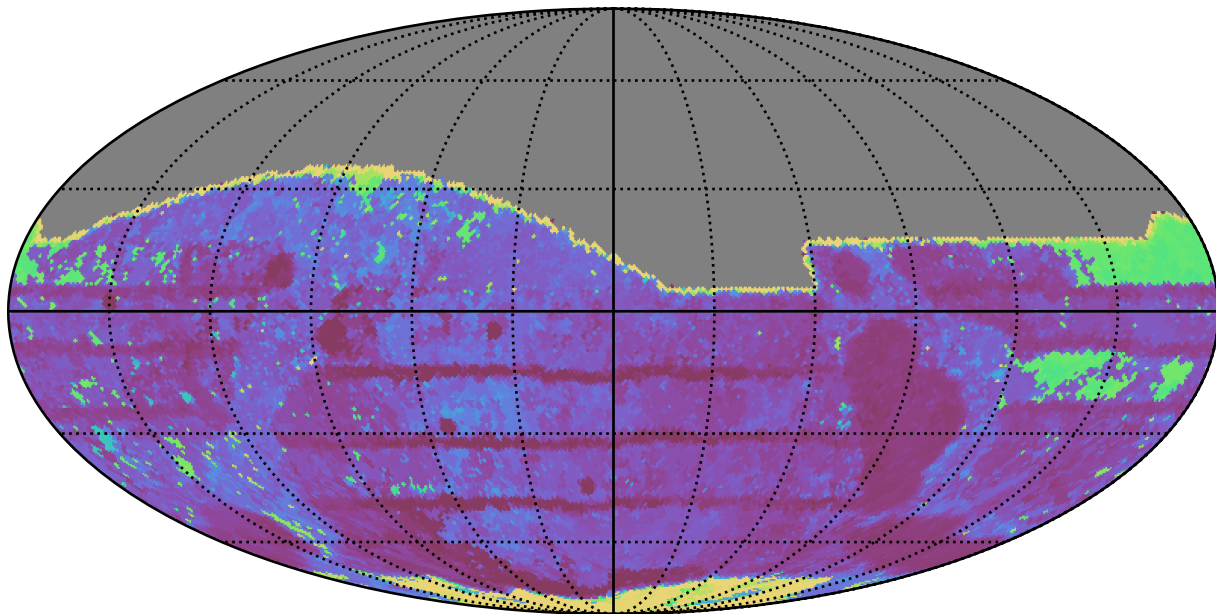
weather_cloudso16v3.4_10yrs All sky r band: Max Inter-Night Gap
