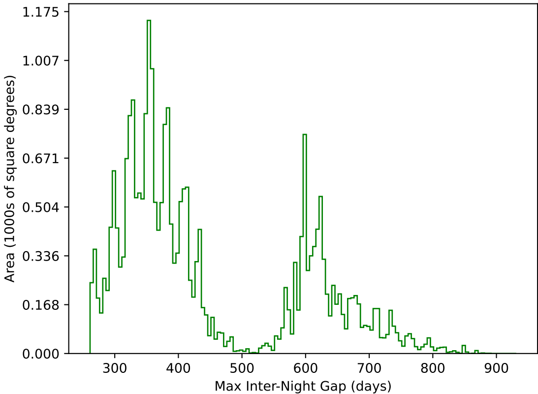
weather_cloudso16v3.4_10yrs All sky g band: Max Inter-Night Gap
