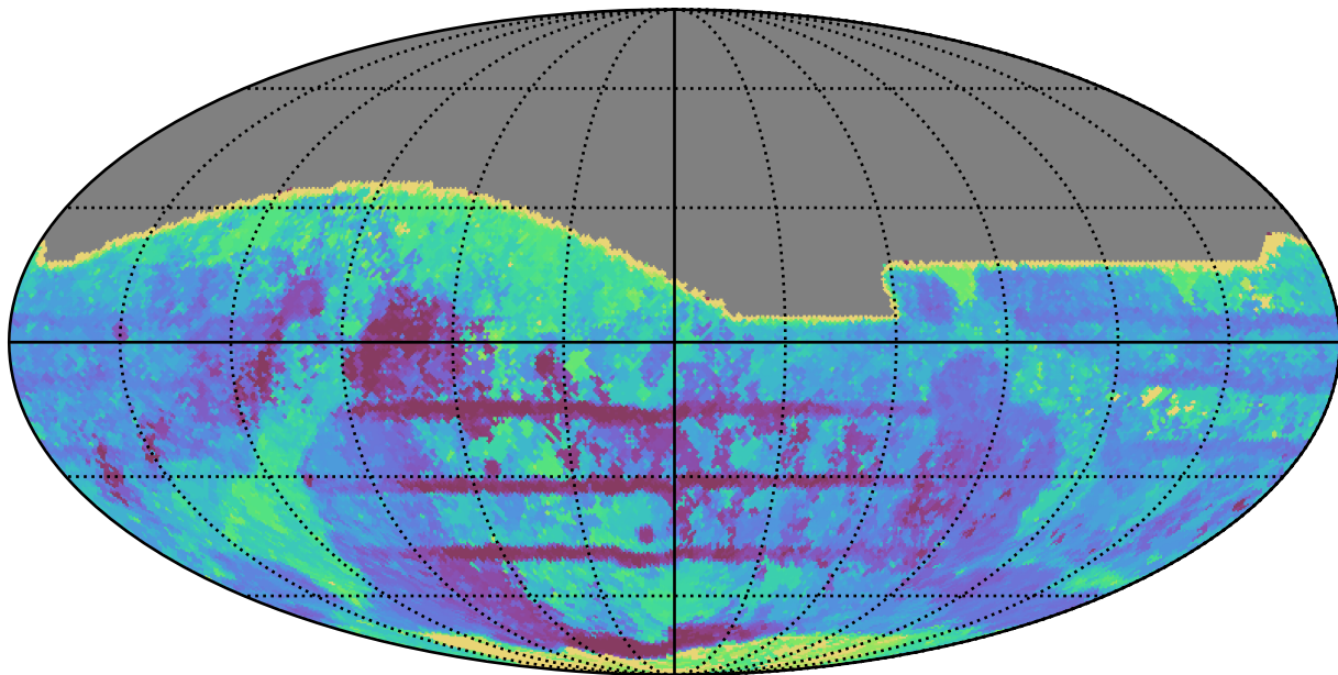
weather_cloudso16v3.4_10yrs All sky all bands: Max Inter-Night Gap
