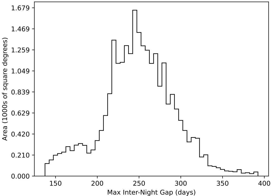
weather_cloudso16v3.4_10yrs All sky all bands: Max Inter-Night Gap
