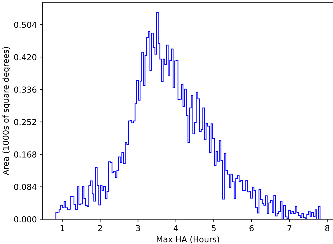
weather_cloudso16v3.4_10yrs All sky u band: Max HA
