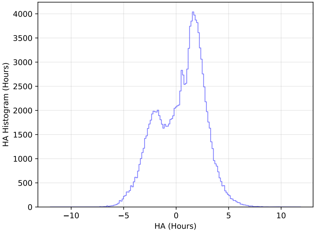
weather_cloudso16v3.4_10yrs WFD u band: HA Histogram
