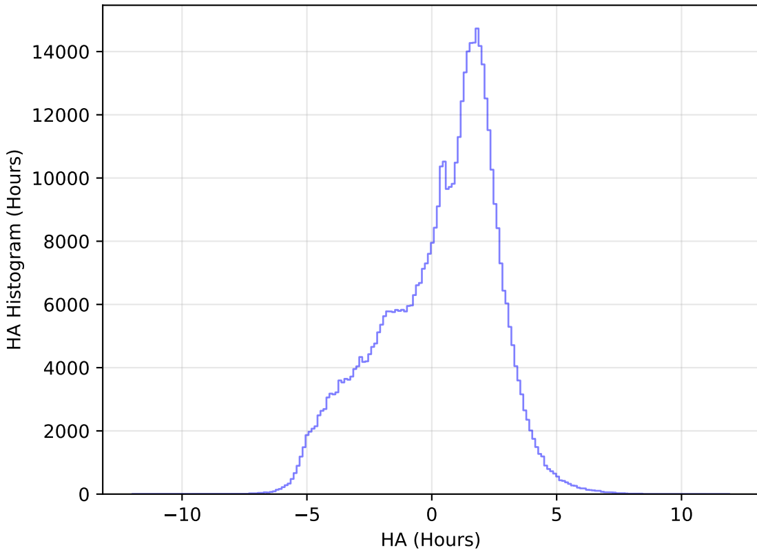
weather_cloudso16v3.4_10yrs WFD r band: HA Histogram
