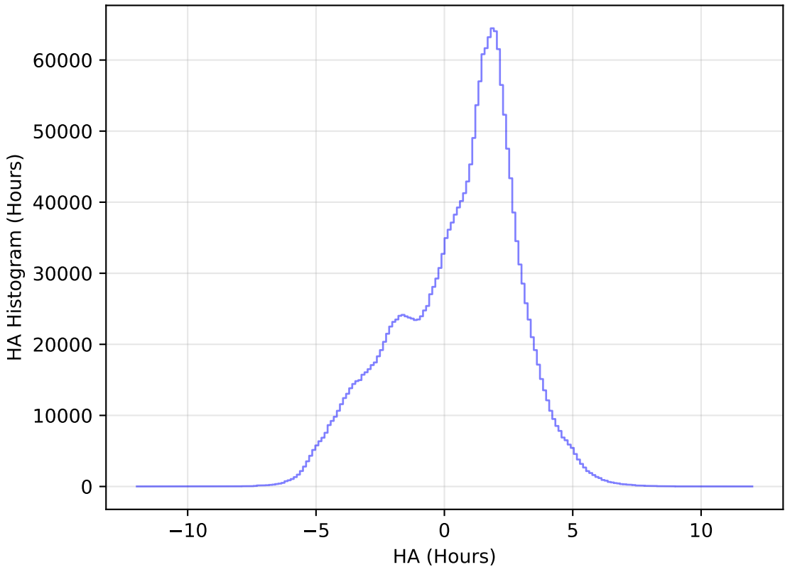
weather_cloudso16v3.4_10yrs WFD all bands: HA Histogram
