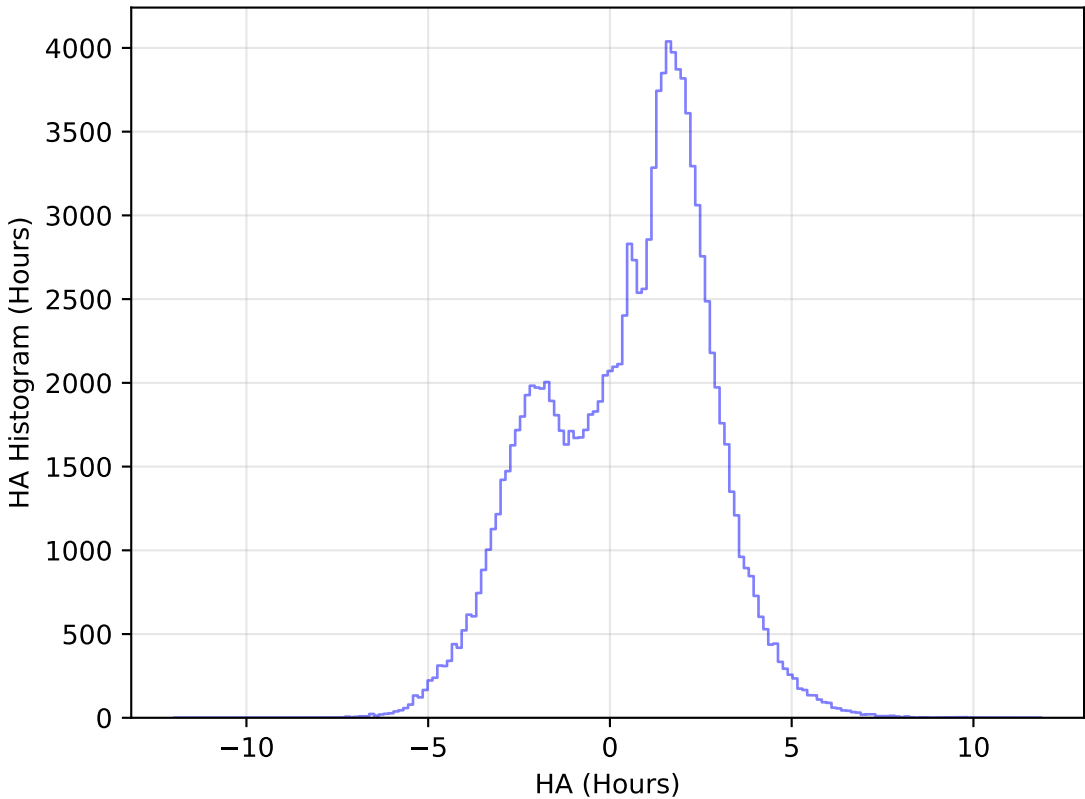
weather_cloudso16v3.4_10yrs All sky u band: HA Histogram
