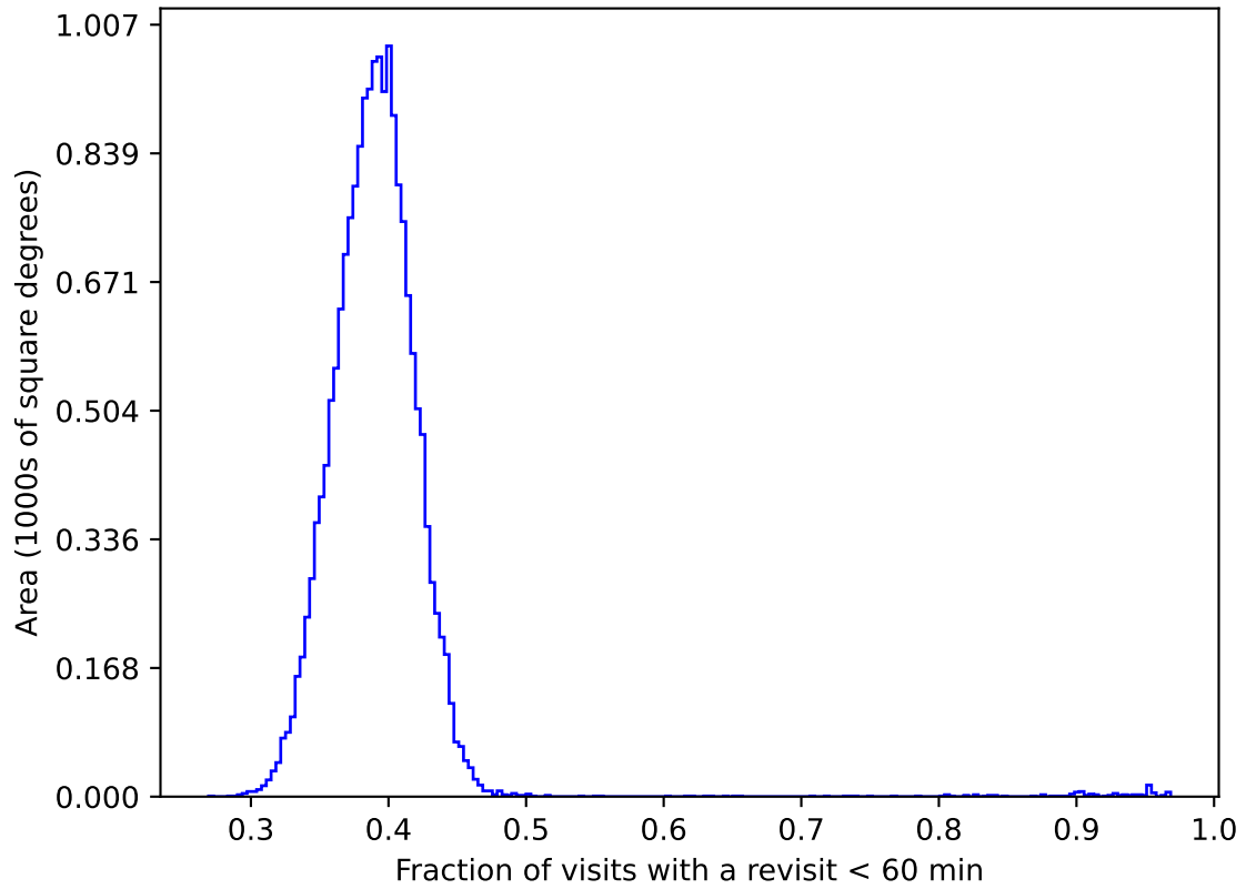
weather_cloudso16v3.4_10yrs gri WFD: Fraction of visits with a revisit < 60 min
