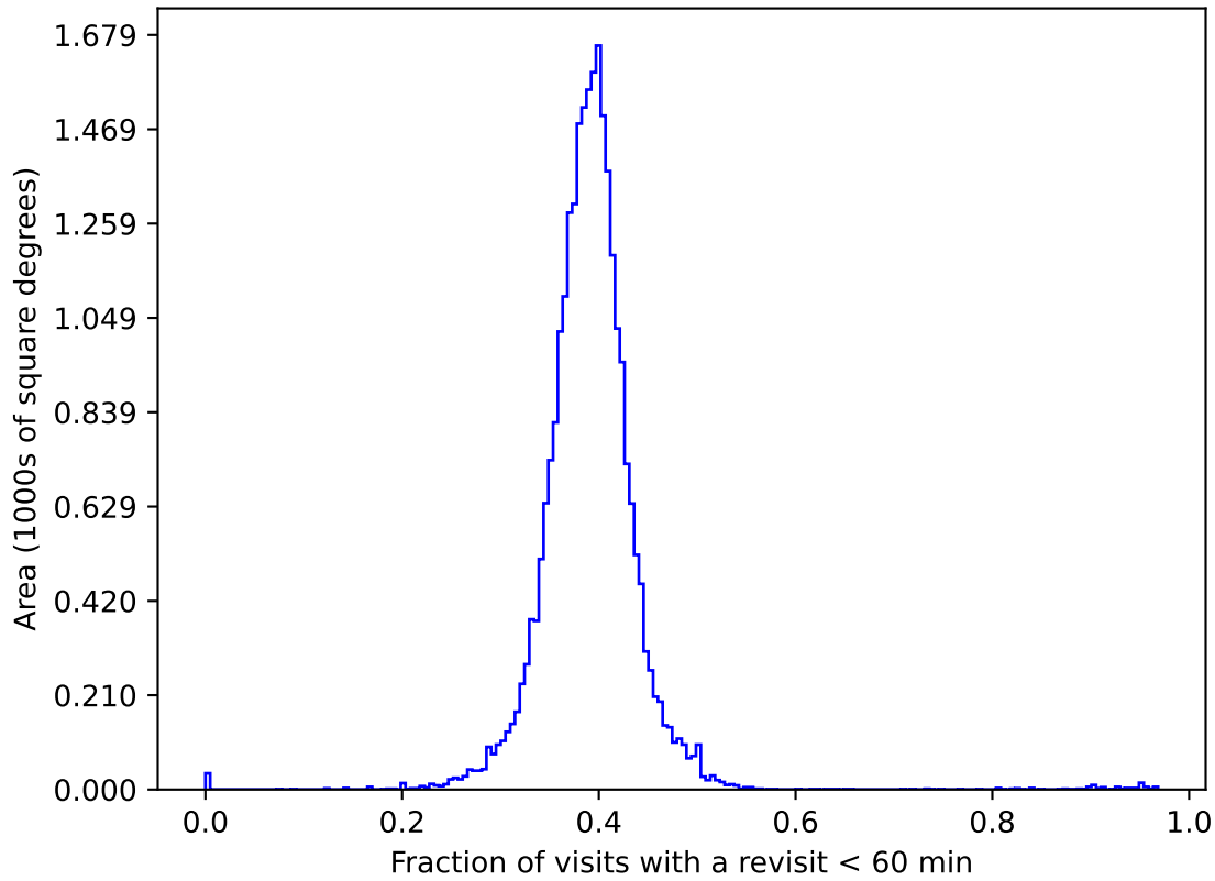
weather_cloudso16v3.4_10yrs gri All sky: Fraction of visits with a revisit < 60 min
