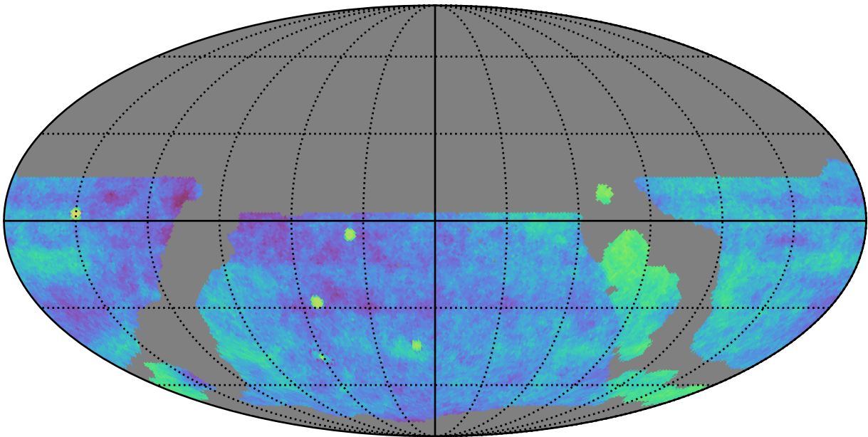
weather_cloudso16v3.4_10yrs gri WFD: Fraction of visits in pairs (20-90 min)
