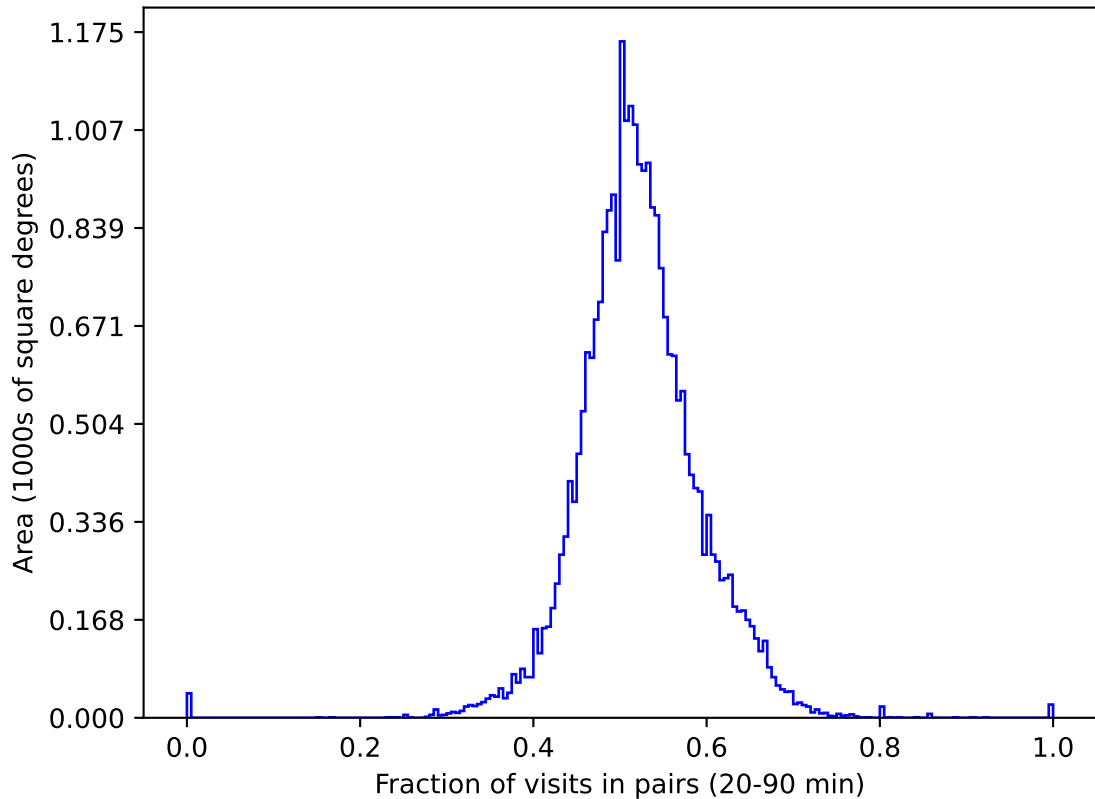
weather_cloudso16v3.4_10yrs gri All sky: Fraction of visits in pairs (20-90 min)
