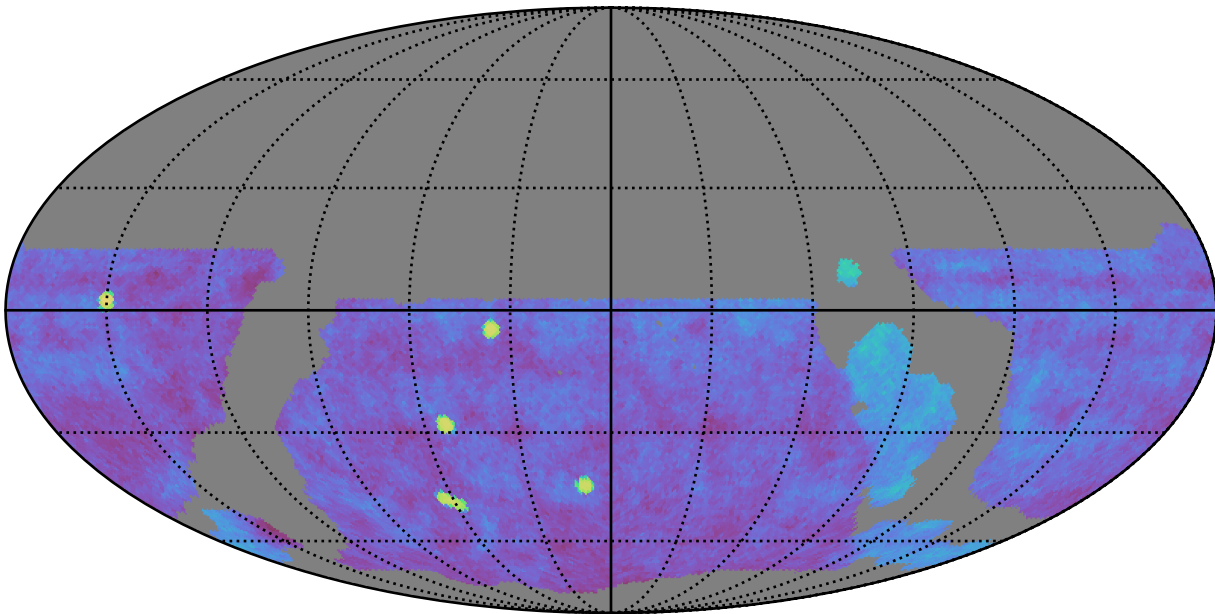
weather_cloudso16v3.4_10yrs gri WFD: Fraction of visits in pairs (10-60 min)
