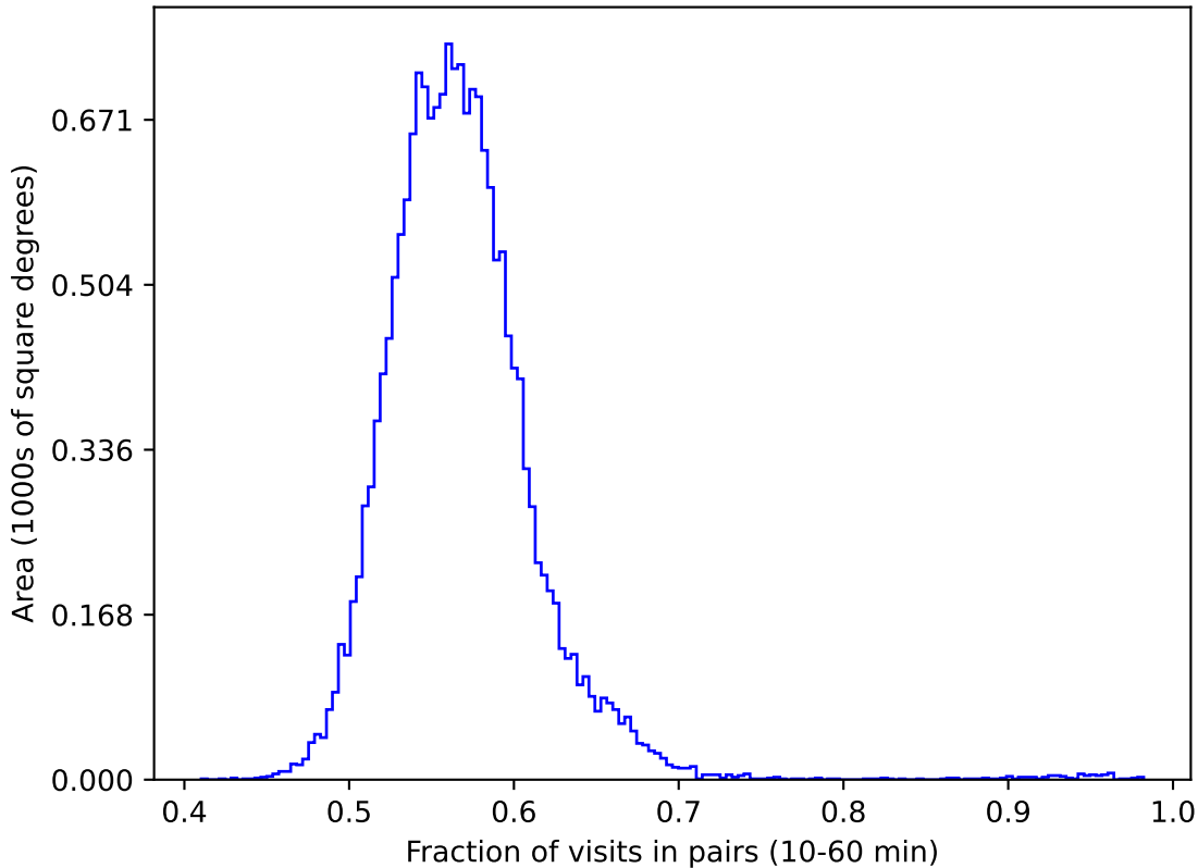
weather_cloudso16v3.4_10yrs gri WFD: Fraction of visits in pairs (10-60 min)
