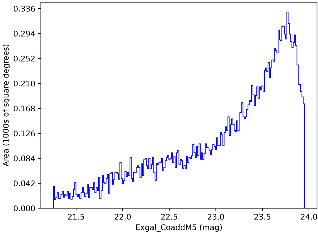
weather_cloudso16v3.4_10yrs Yr 3-4 y band: Exgal_CoaddM5
