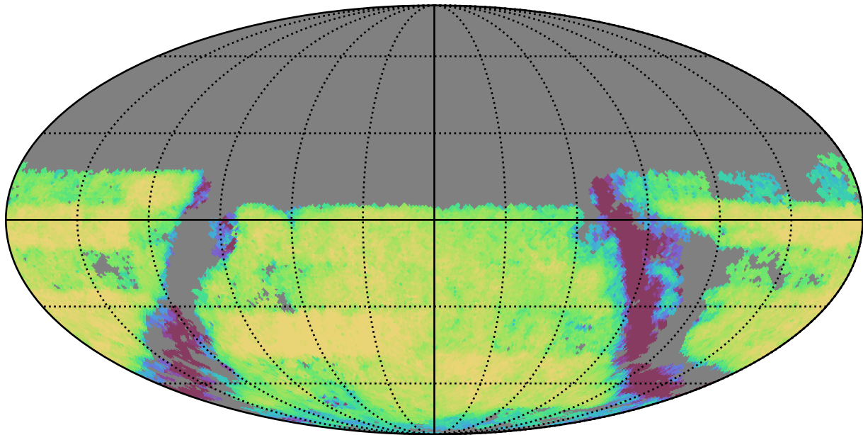
weather_cloudso16v3.4_10yrs Yr 3-4 u band: Exgal_CoaddM5
