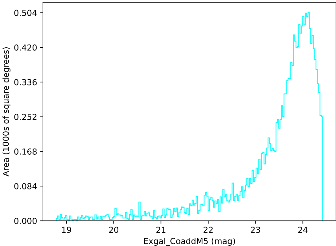
weather_cloudso16v3.4_10yrs Yr 3-4 u band: Exgal_CoaddM5
