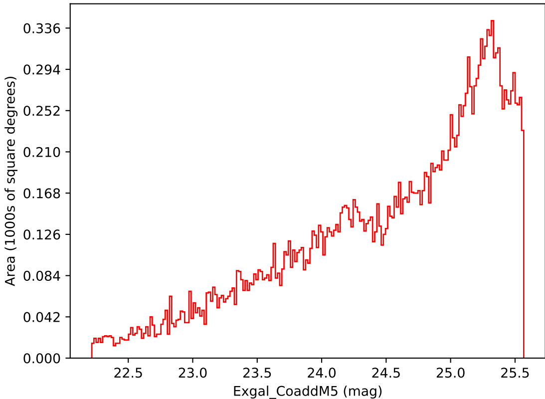
weather_cloudso16v3.4_10yrs Yr 3-4 i band: Exgal_CoaddM5
